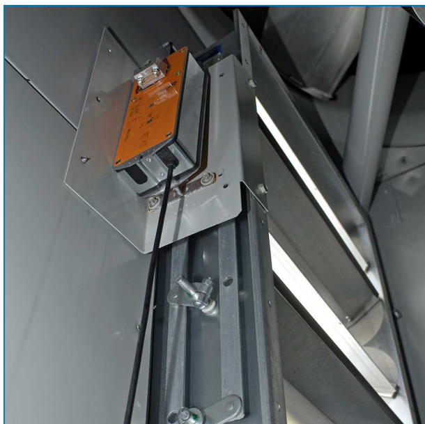
Actuator for modulating air inlet dampers
