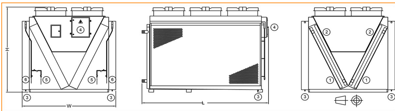
1. Fluid inlet connection; 2. Fluid outlet connection; 3. Pre-cooler water drain; 4. Electrical panel; 5. Pre-cooler city water connection; 6. Pre-cooler pad.
