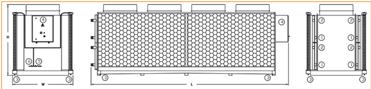
1. Fluid inlet connections; 2. Fluid outlet connections; 3. Pre-cooler water drain; 4. Electrical panel; 5. Pre-cooler city water connection; 6. Pre-cooler piping drain.
