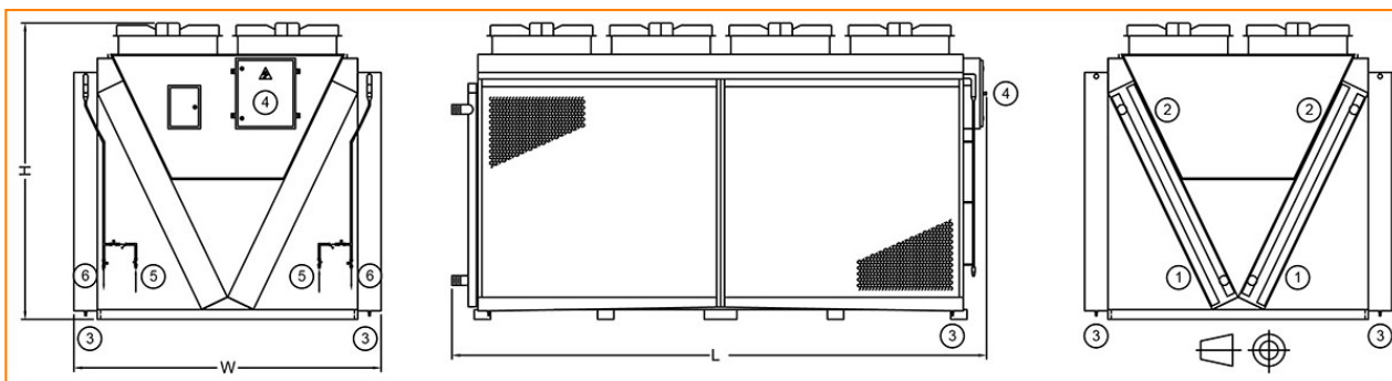
1. Fluid inlet connection; 2. Fluid outlet connection; 3. Pre-cooler water drain; 4. Electrical panel; 5. Pre-cooler city water connection; 6. Pre-cooler pad.
